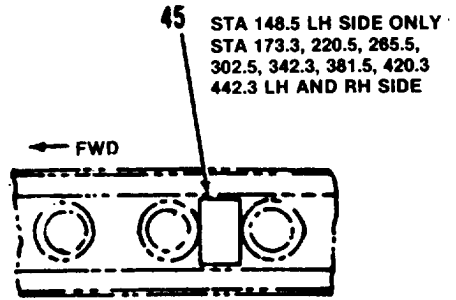
DETAIL G
