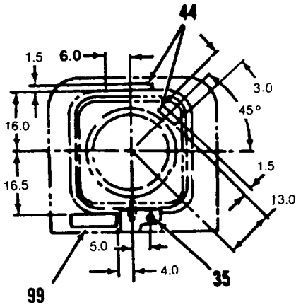
DETAIL H (LOOKING OUTBD)
