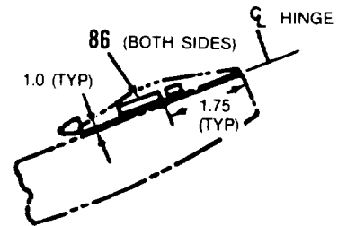
VIEW T-T
